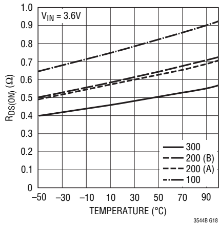
PFET R_{DS(ON)} vs Temperature
